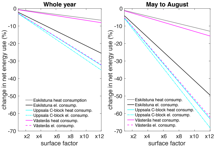
Figure 4.8. The effect on energy use in the WWTPs by changing the surface size of the microalgae-bacteria basin
