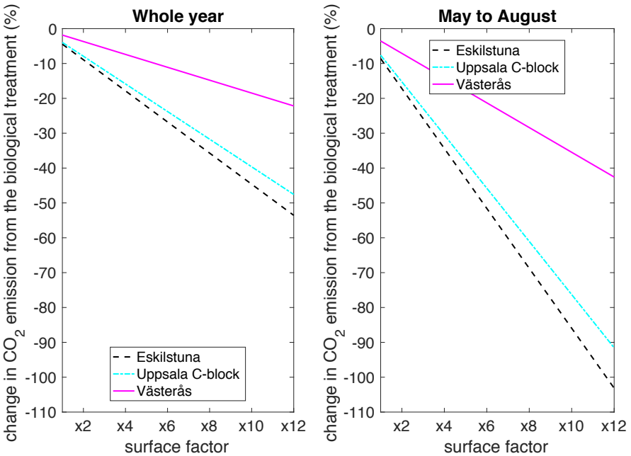
Figure 4.9. The effect on the carbon dioxide emissions in the WWTPs by changing the surface size of the microalgae-bacteria basin
